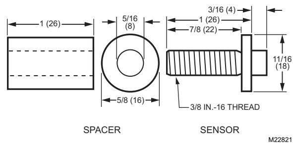
Fig. 2. Dimensions of C7021P, C7023P, C7041P in in. (mm)
