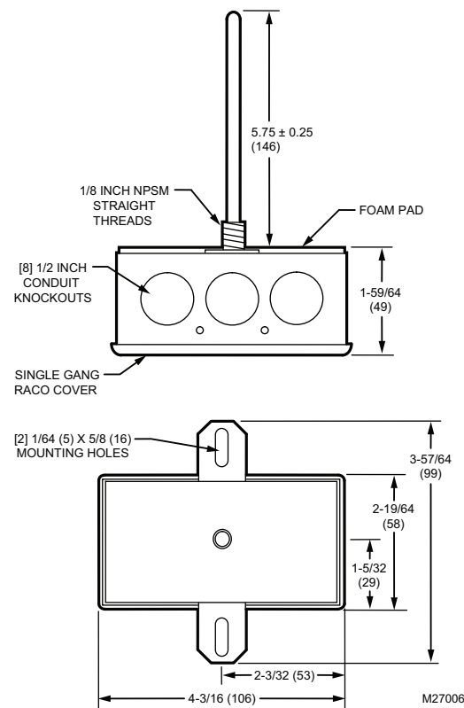
Fig. 3. C7031B dimensions in in. (mm)
