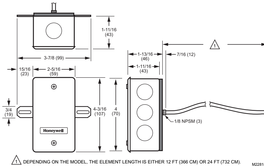
Fig. 7. C7021R, C7023R, C7041R dimensions in in. (mm).
