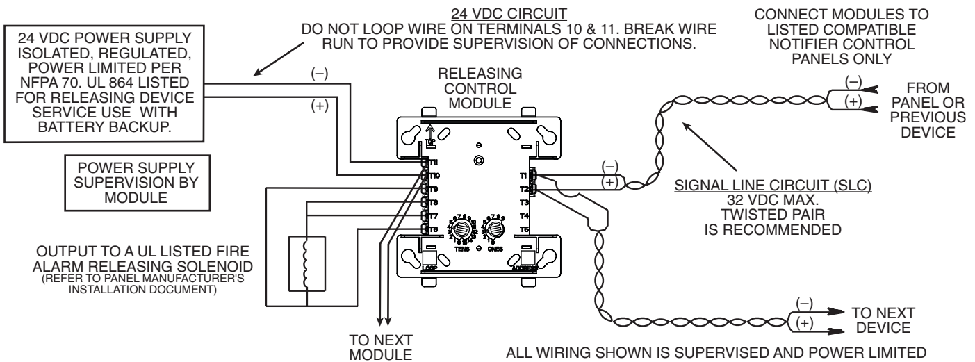
FIGURE 4. TYPICAL CLASS A, SOLENOID CONFIGURATION:
