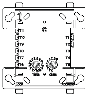
FIGURE 1A. CONTROLS AND INDICATORS:
