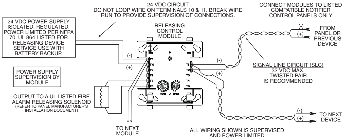
FIGURE 3. TYPICAL CLASS B, SOLENOID CONFIGURATION:
