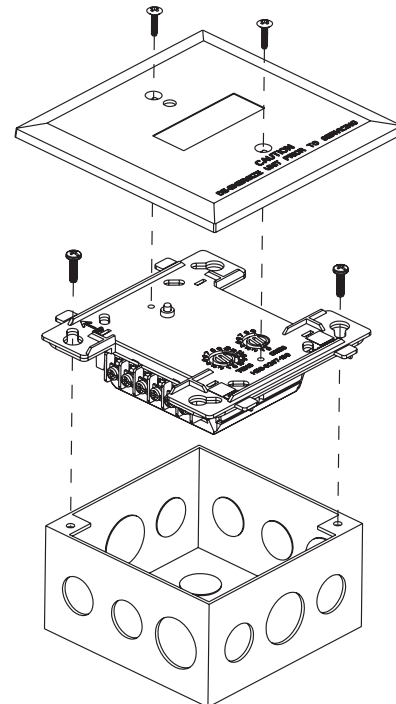
FIGURE 2. MODULE MOUNTING:
