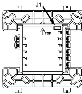
FIGURE 1B. JUMPER LOCATION:
