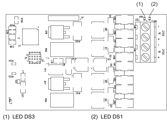
Figura 1: Diodos LED de la tarjeta FX-SLC1
