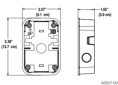
Compact Surface Mount Back Box for Walls (SBBGRL, SBBGWL)
