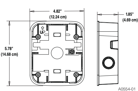
Surface Mount Back Box for Walls ( SBBRL/SBBWL)
