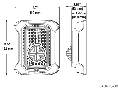
Strobes, Horn Strobes for Walls
